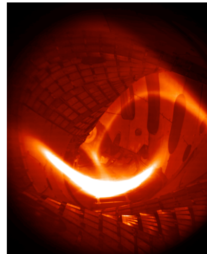
Figure 1. Helically twisted plasma glows during the first hydrogen operation in W7-X on Feb. 3, 2016. [Photo: IPP]
