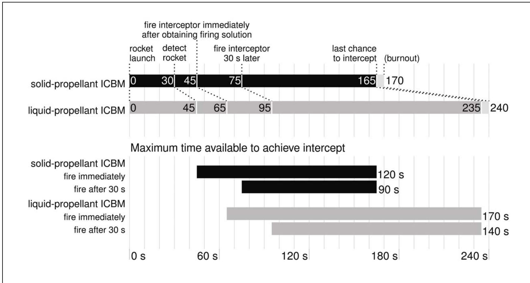
Figure 2.2: ICBMs would need to be engaged on a very compressed timeline. The upper half of the figure shows the stages of the intercept process for both solid- and liquid-propellant ICBMs launched from Iran. The right hand end of the solid bars indicates when the ICBM stops burning. The last chance for intercepting the ICBM is five seconds before that, as indicated.
