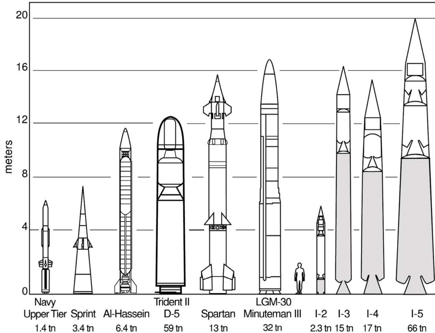
Figure 16.9: Comparison of hypothetical model interceptors with various existing missiles. The estimated liftoff mass of each interceptor in tonnes (1 tn = 1000 kg) is listed beneath the name of the interceptor or missile. Interceptors I-2, I-3, I-4 and I-5 are hypothetical interceptors modeled in the report.
