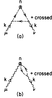
FIG. 5. Contributions to {}^n\gamma_{VV}^G . The coefficients of g_{\mu\nu} arise from diagram (a).
