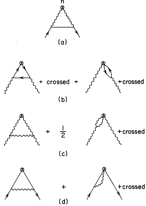
FIG. 2. Graphs for computing \underline{\gamma} (radiative corrections to matrix elements). (a) The matrix element of {}^n O^V between fermion states. (b) The matrix element of {}^n O^F between vector states. (c) The matrix element of {}^n O^V between vector states. (d) The matrix element of {}^n O^F between fermion states.
