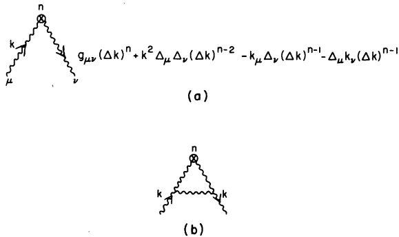
FIG. 3. Graphs for computing \gamma_{VV}^V in quantum electrodynamics in the gauge of Eq. (A1). (a) The vertex for {}^V O^{(n)} . (b) The radiative correction to the matrix element of {}^V O^{(n)} between vector states.
