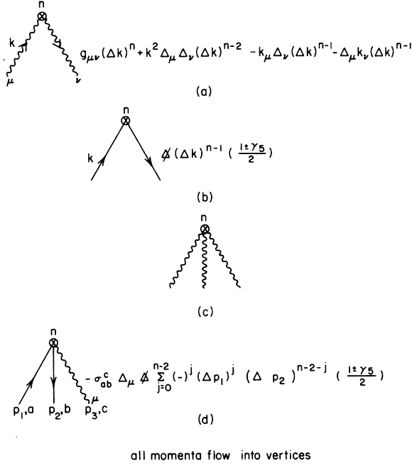
FIG. 1. (a) The vertex for {}^n O^V (order 0). (b) The vertex for {}^n O^F (order 0). (c) The vertex for {}^n O^V (order g ). (d) The vertex for {}^n O^F (order g ).
