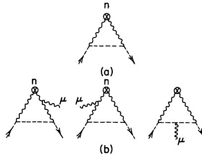
FIG. 4. Mixing of vector and ghost operators. (a) The zero-order contributions to {}^G O^{(n)} . (b) The order- g contributions to {}^G O^{(n)} .
