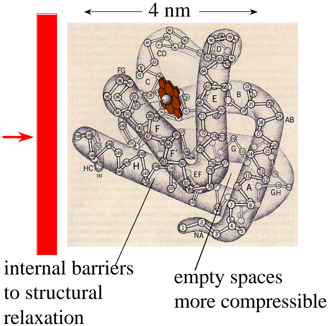
Fig. 1 Shock wave compression of a protein.
